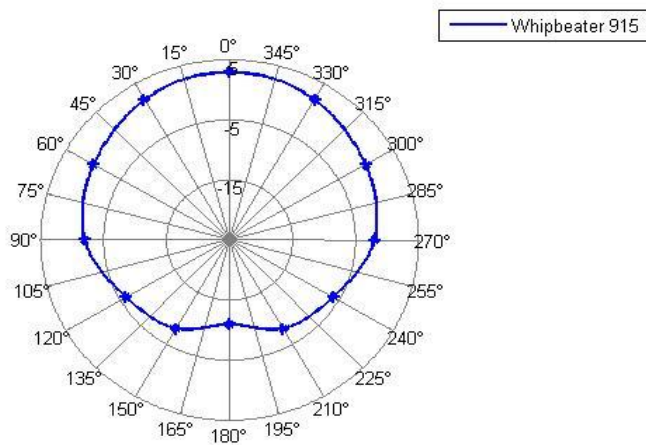
Azimuthal power pattern. DBi values when Internally Mounted at 915MHz
